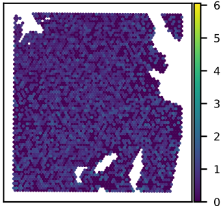
SNU51A POMT1 expression Moran's I = 0.01
