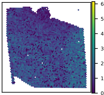
SNU27A ALDOC expression Moran's I = 0.25
