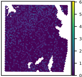
SNU51A RENBP expression Moran's I = 0.07
