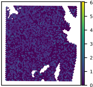
SNU51A SLC25A32 expression Moran's I = 0.02
