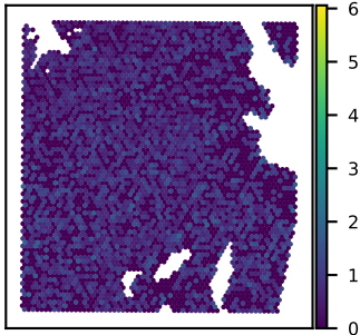
SNU51A SRCAP expression Moran's I = 0.02
