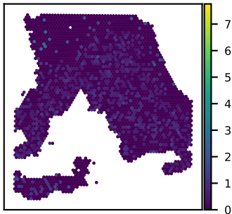
SNU18A MAP3K1 expression Moran's I = 0.04
