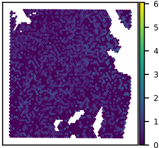
SNU51A KCTD1 expression Moran's I = 0.04
