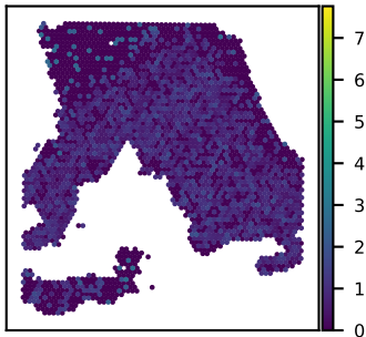
SNU18A SLC35F5 expression Moran's I = 0.09
