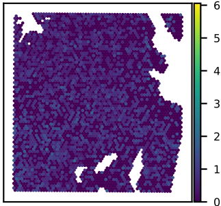
SNU51A DCP2 expression Moran's I = 0.03
