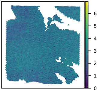
SNU24B HNRNPA2B1 expression Moran's I = 0.27
