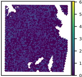
SNU51A VAMP5 expression Moran's I = 0.02
