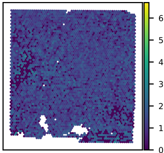
SNU43A SSBP1 expression Moran's I = 0.05
