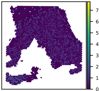
SNU18A C1orf216 expression Moran's I = 0.05
