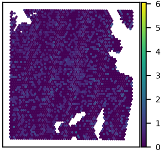
SNU51A KIAA1586 expression Moran's I = 0.01
