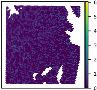
SNU51A CENPC expression Moran's I = 0.03
