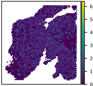
SNU24A PCSK1N expression Moran's I = 0.05
