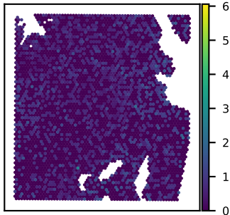
SNU51A MROH1 expression Moran's I = 0.03
