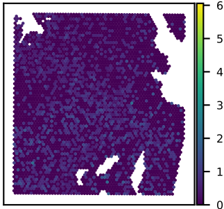
SNU51A TRAIP expression Moran's I = 0.05
