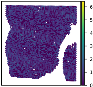
SNU25B RCAN1 expression Moran's I = 0.01
