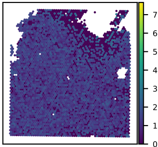
SNU21B PSMA2 expression Moran's I = 0.08
