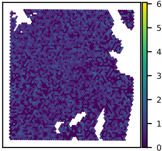
SNU51A CWC15 expression Moran's I = 0.01
