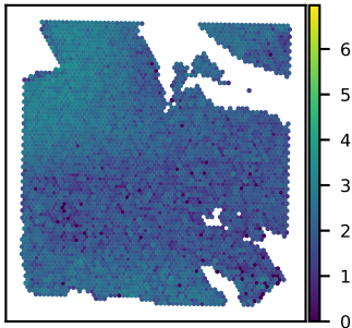
SNU24B SLC22A17 expression Moran's I = 0.48
