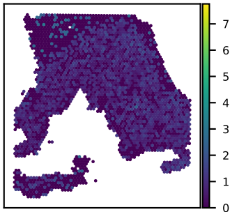
SNU18A TP53RK expression Moran's I = 0.09
