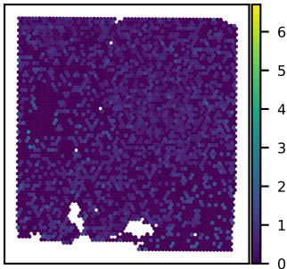
SNU43A ARHGAP33 expression Moran's I = 0.02
