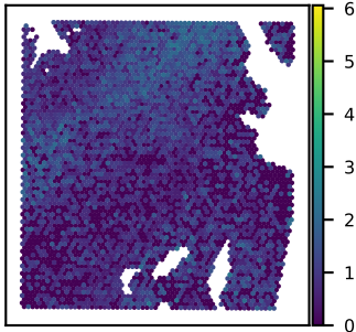
SNU51A CAPG expression Moran's I = 0.28
