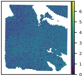
SNU24B SNRNP70 expression Moran's I = 0.22
