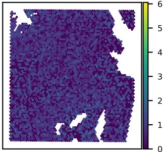
SNU51A MKNK2 expression Moran's I = 0.01
