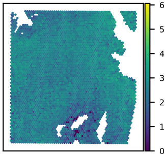
SNU51A SLC1A3 expression Moran's I = 0.47
