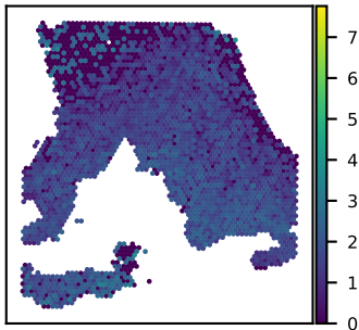
SNU18A BAALC expression Moran's I = 0.27
