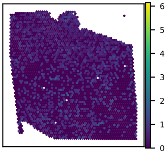
SNU27A C1orf162 expression Moran's I = 0.04
