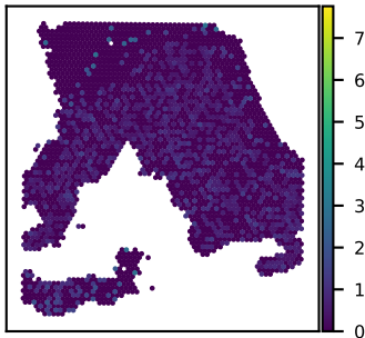
SNU18A CENPC expression Moran's I = 0.03
