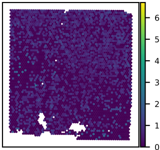
SNU43A CREB3L2 expression Moran's I = 0.05
