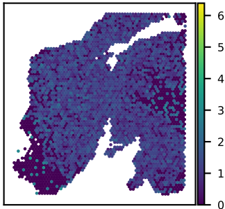
SNU24A ADAM9 expression Moran's I = 0.15
