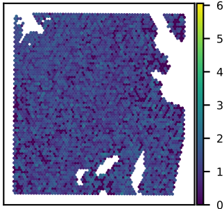
SNU51A PPP1R15B expression Moran's I = 0.03
