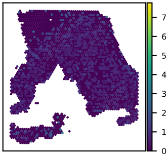
SNU18A FBRSL1 expression Moran's I = 0.04
