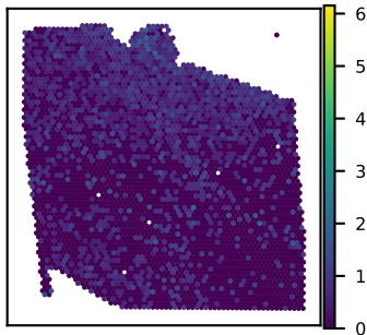
SNU27A ADAP2 expression Moran's I = 0.20
