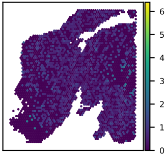
SNU24A PTPDC1 expression Moran's I = 0.05
