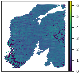
SNU24A ARGLU1 expression Moran's I = 0.07
