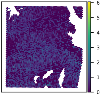
SNU51A MELK expression Moran's I = 0.15
