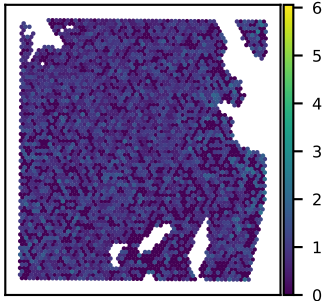
SNU51A SNRNP25 expression Moran's I = 0.02
