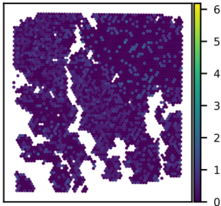
SNU16B TMEM216 expression Moran's I = 0.02
