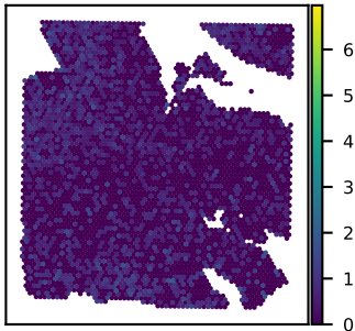
SNU24B SEPTIN6 expression Moran's I = 0.09
