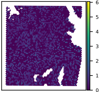
SNU51A RPUSD1 expression Moran's I = 0.02
