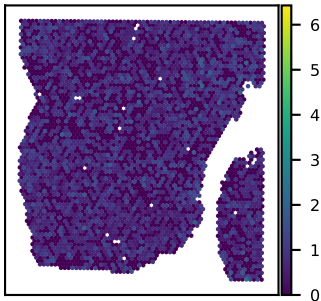
SNU25B SLC35A5 expression Moran's I = 0.02
