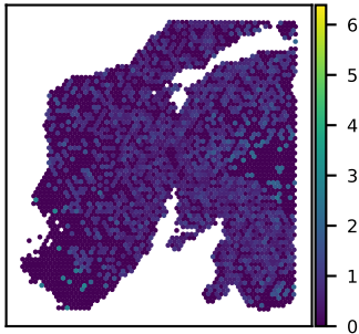
SNU24A EMILIN1 expression Moran's I = 0.05
