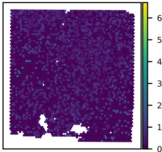
SNU43A TMCC1 expression Moran's I = 0.02
