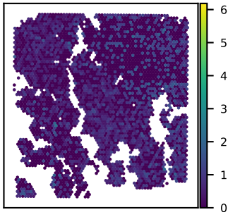
SNU16B LHFPL2 expression Moran's I = 0.05
