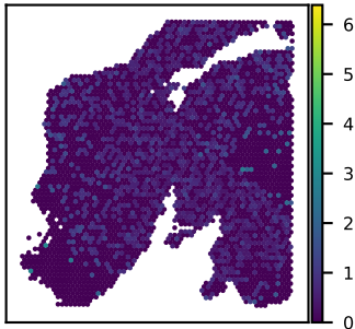
SNU24A ATG2A expression Moran's I = 0.04
