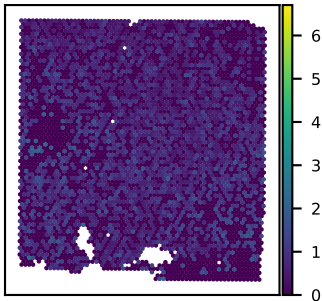
SNU43A C11orf98 expression Moran's I = 0.05
