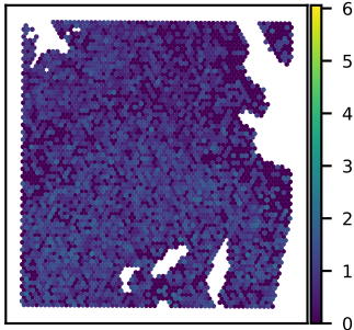
SNU51A PCGF2 expression Moran's I = 0.10
